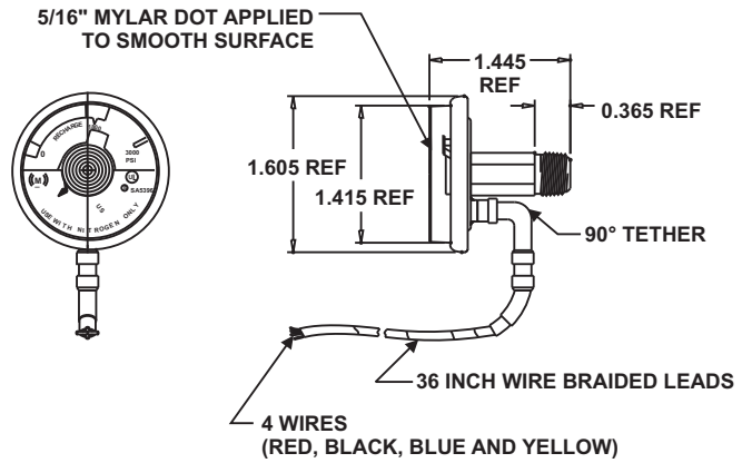
Figure 1. Switch-in-Gauge Dimensions
